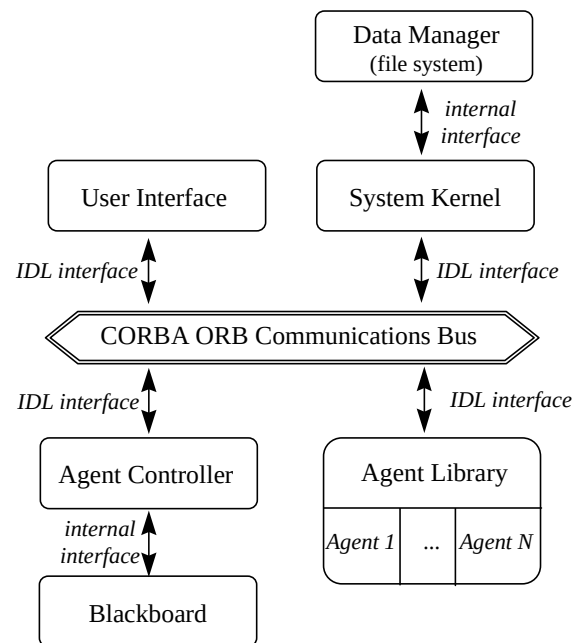
Figure 3 Component Architecture
