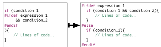
Figure 9: A generic refactoring for if statements.
