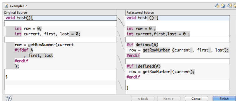
Figure 6: Colligens view to refactor incomplete annotations.
