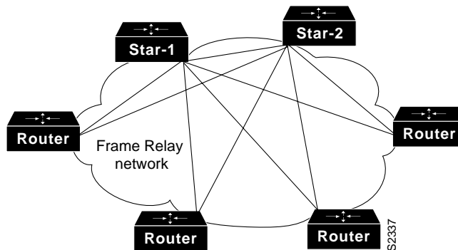
Figure 9-8 Twin-Star Partially Meshed Frame Relay Internetwork
