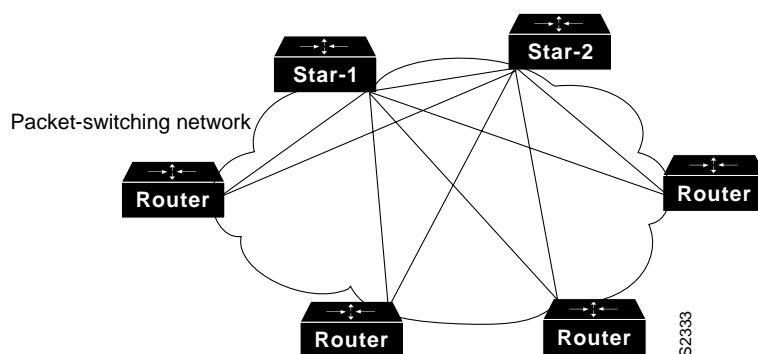
Figure 9-1 Hierarchical Packet-Switched Interconnection
