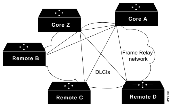
Figure 9-9 Partially Meshed Frame Relay Internetwork
