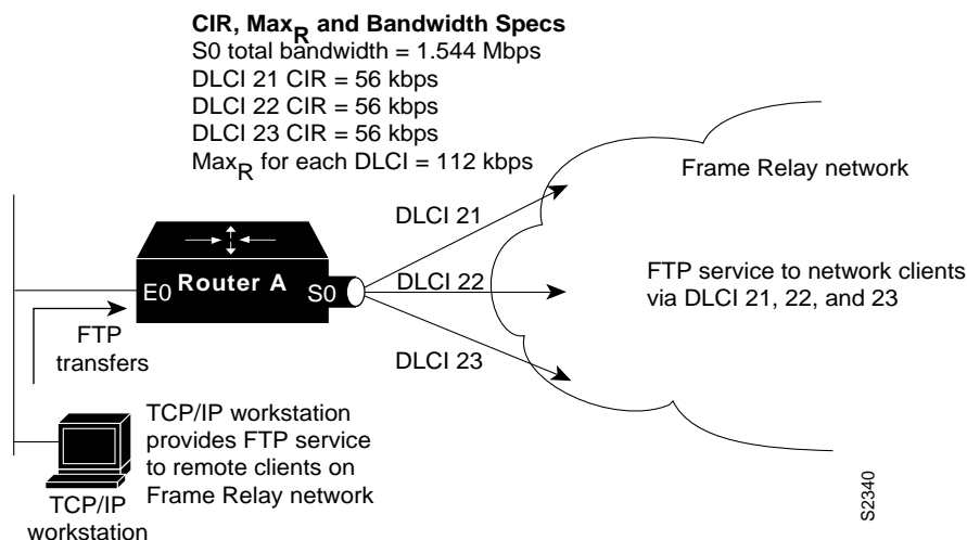
Figure 9-11 Example of a CIR and CBR Traffic Limiting Situation
