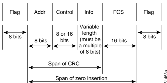
Figure 5-2 SDLC Frame Format
