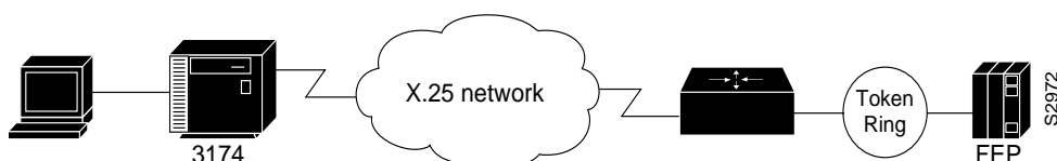
Figure 5-18 Simple Topology for QLLC Conversion
