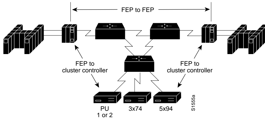
Figure 5-1 Sample STUN Network Configuration
