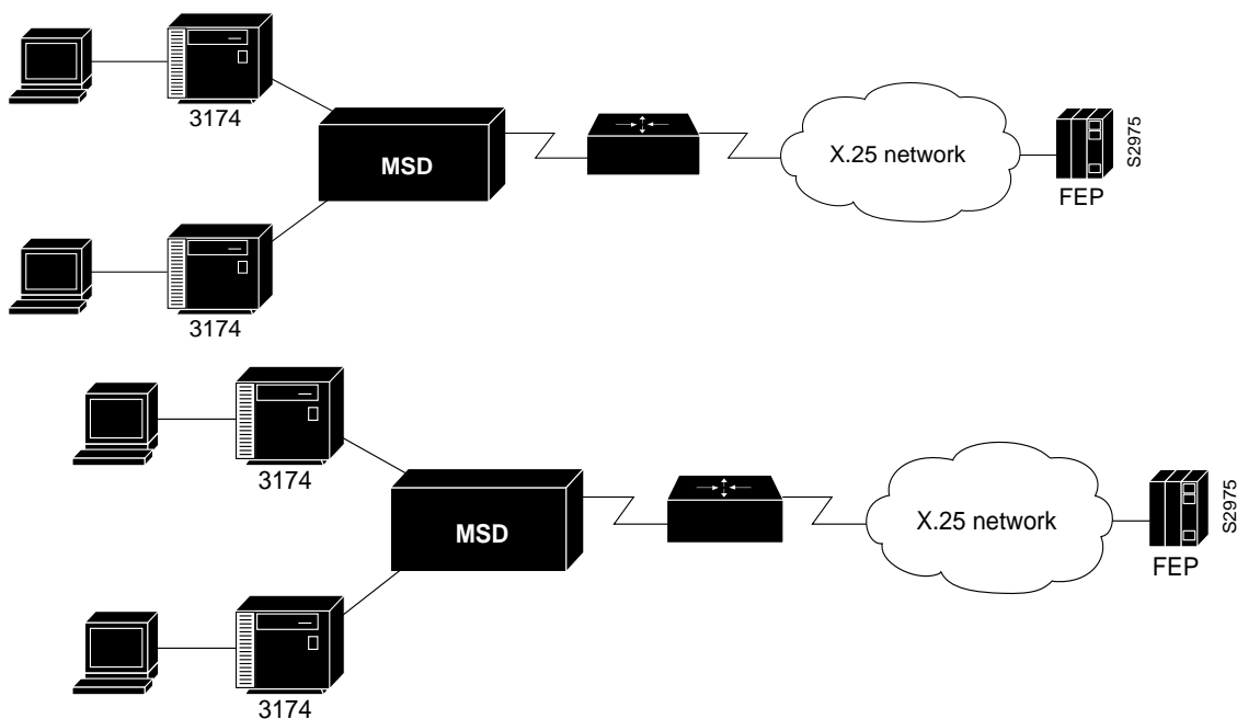
Figure 5-20 QLLC Conversion Supports Multidrop SDLC Topology
