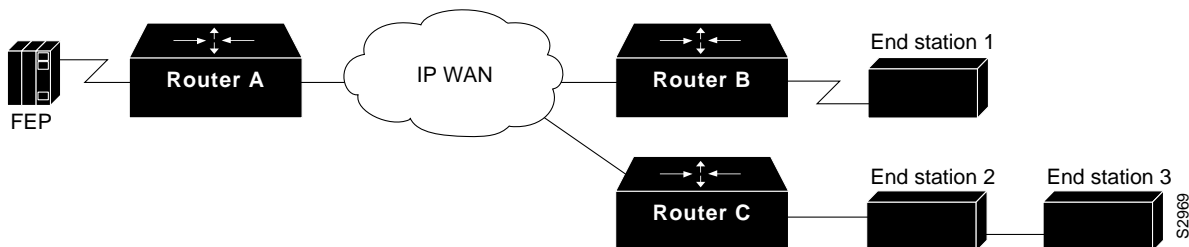
Figure 5-5 SDLC Broadcast in Virtual Multidrop Line Environment
