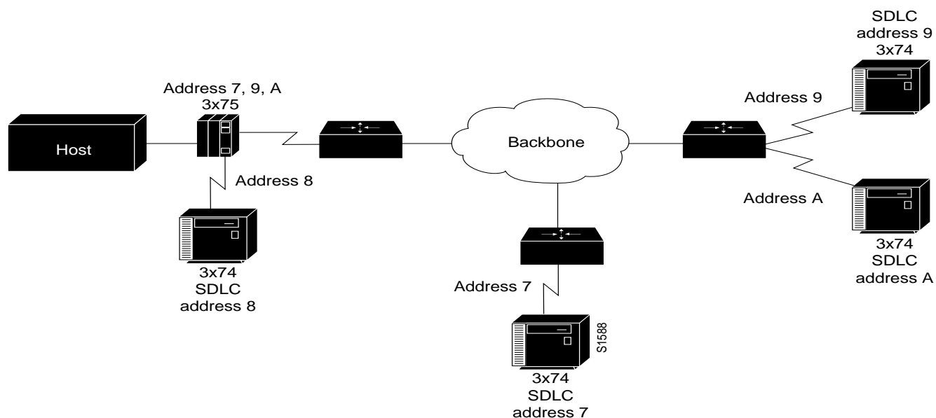
Figure 5-4 SDLC Transport in Virtual Multidrop Environment
