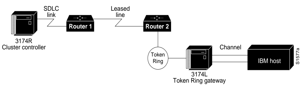
Figure 5-13 SDLLC Implementation with 3174 Token Ring Gateway
