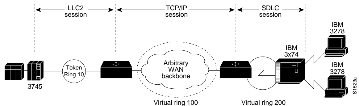
Figure 5-11 Local Acknowledgment Operation
