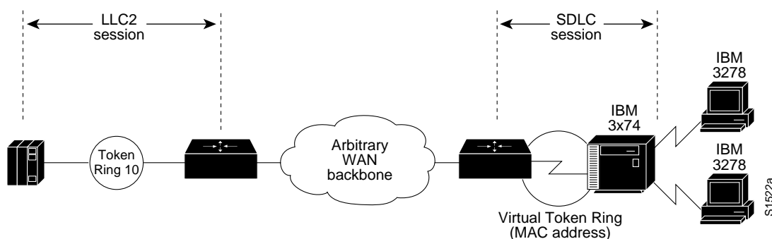
Figure 5-10 SDLLC Media Translation
