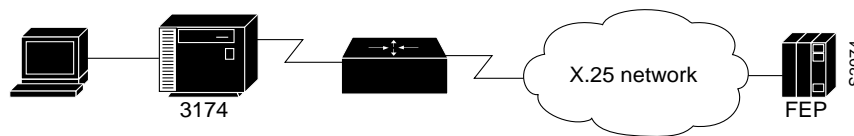
Figure 5-19 Topology that Uses SDLC and QLLC Conversion
