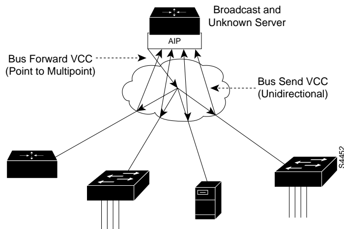
Figure 8-15 BUS Connections
