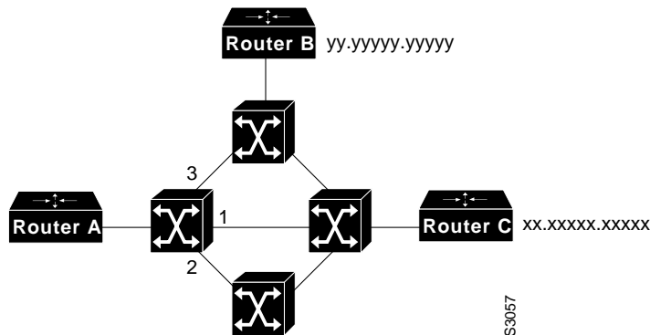
Figure 8-28 Example of a Multiswitch Network That Uses the PNNI Phase 0 Protocol
