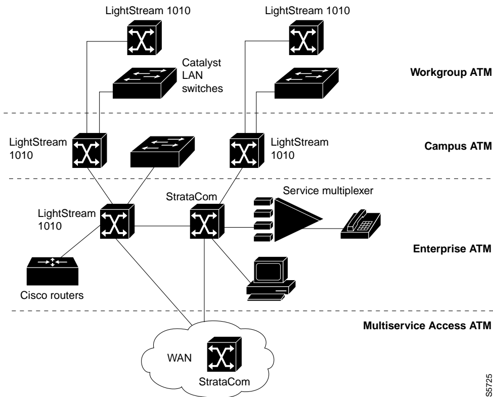
Figure 8-2 Role of ATM Switches in an Internetwork
