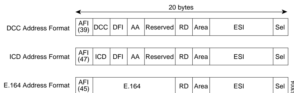
Figure 8-8 ATM Address Formats
