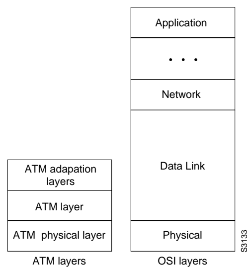
Figure 8-5 Relationship of ATM Functional Layers to the OSI Reference Model
