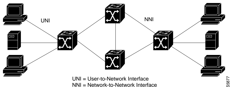
Figure 8-3 Components of an ATM Network
