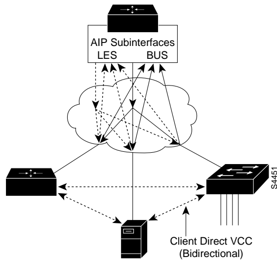
Figure 8-16 Fully Connected ELAN
