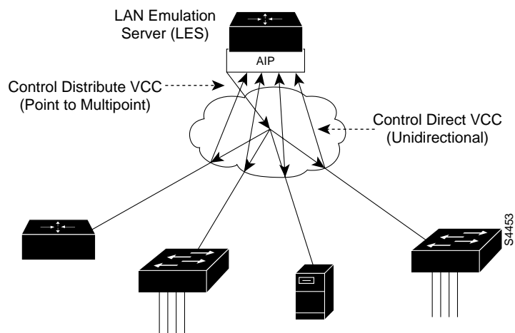
Figure 8-14 LAN Emulation Server (LES) Connections
