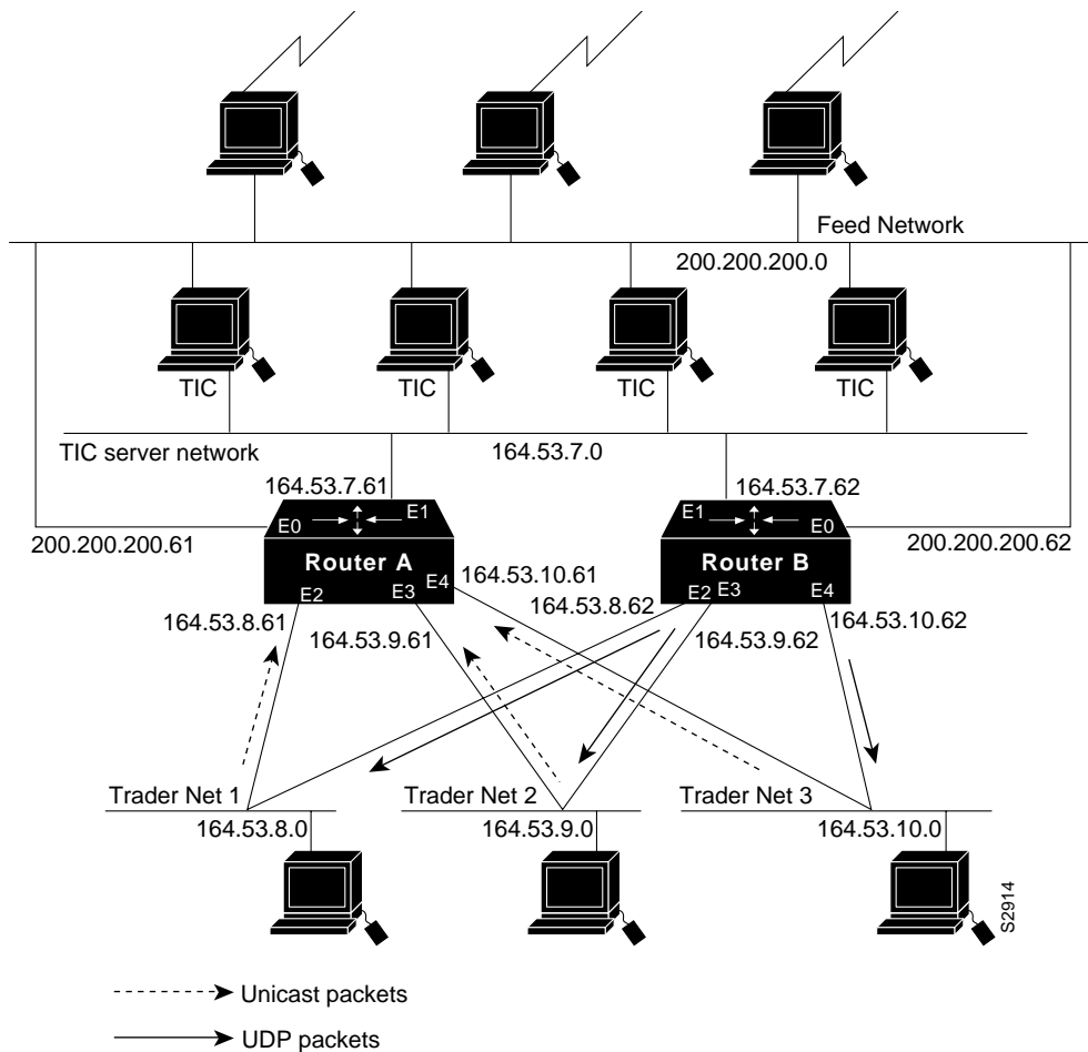
Figure 6-3 Data Flow with UDP Flooding and IRDP
