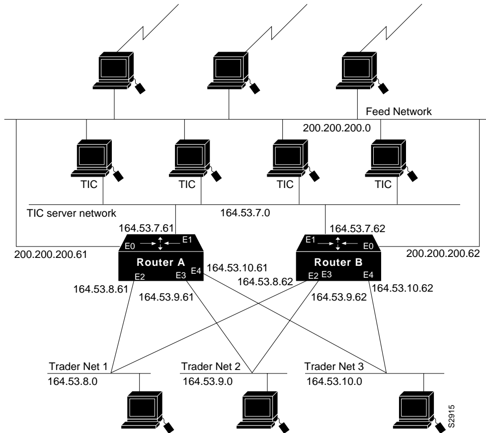
Figure 6-1 Topology That Requires UDP Broadcast Forwarding
