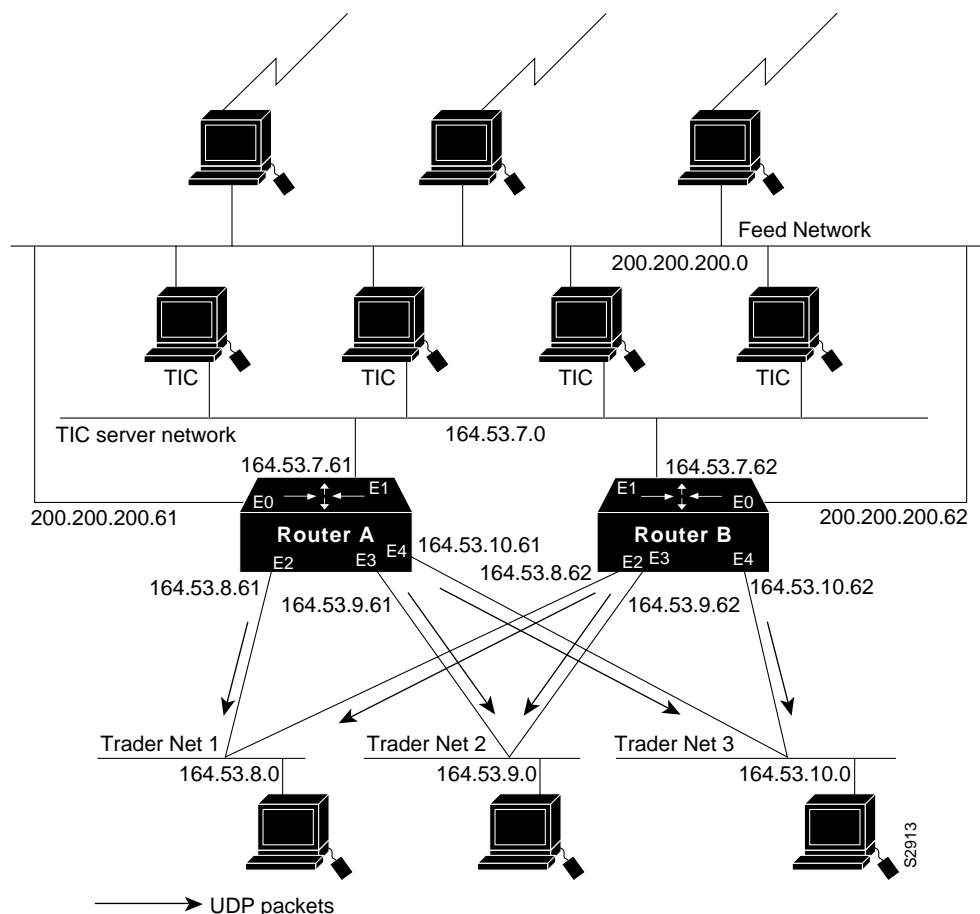
Figure 6-2 Flow of UDP Packets from Routers to Trader Networks Using IP Helper Addressing
