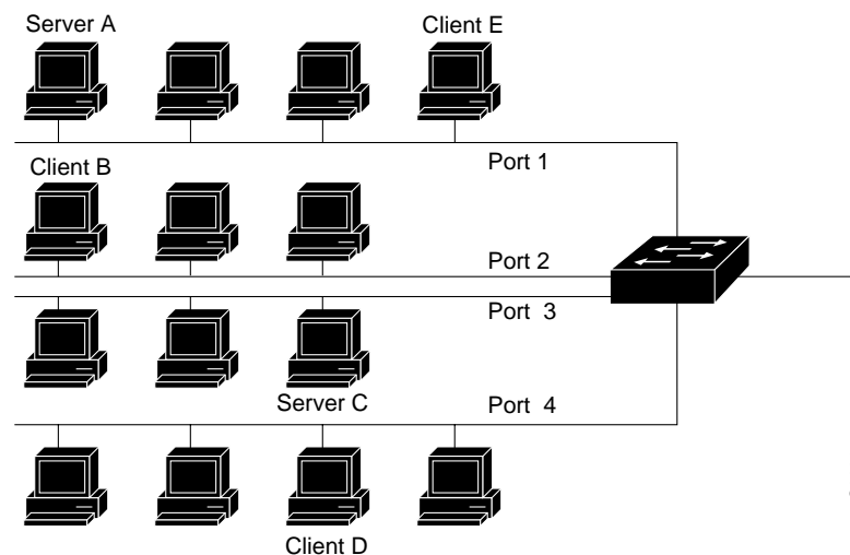
Figure 10-1 Ethernet Switching
