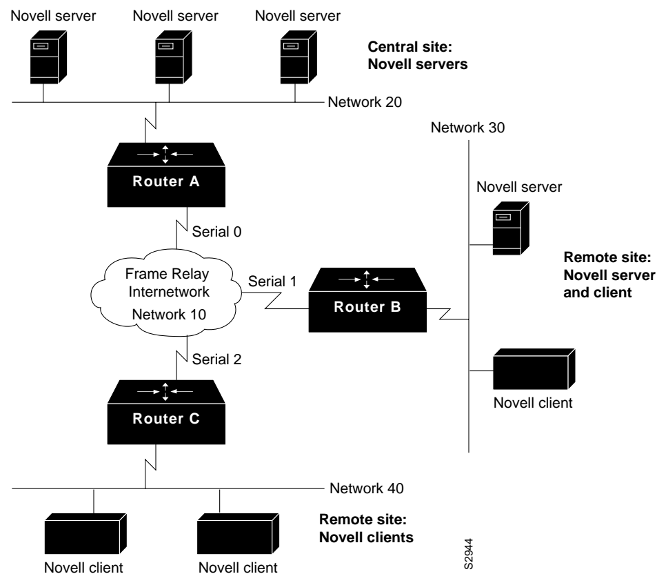
Figure 5-1 Large-Scale Novell IPX Internetwork
