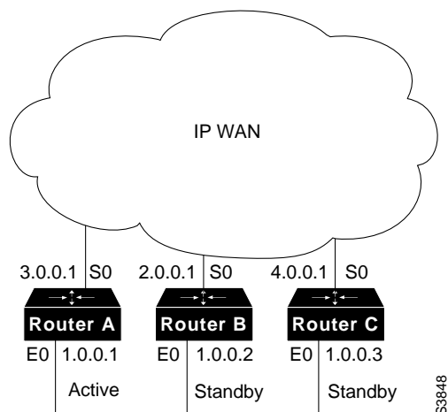
Figure 9-5 Tracking Example
