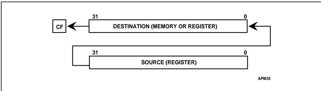
Figure 4-9. SHLD Instruction
