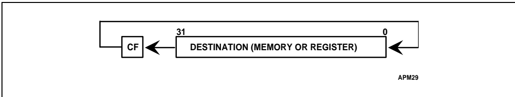
Figure 4-13. RCL Instruction
