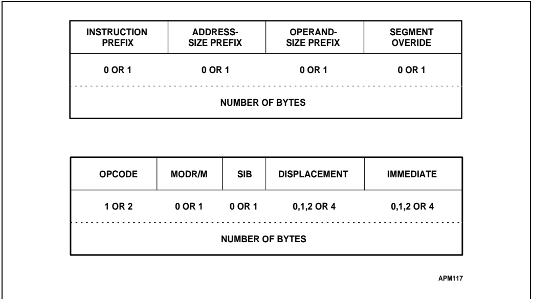
Figure 25-1. Instruction Format
