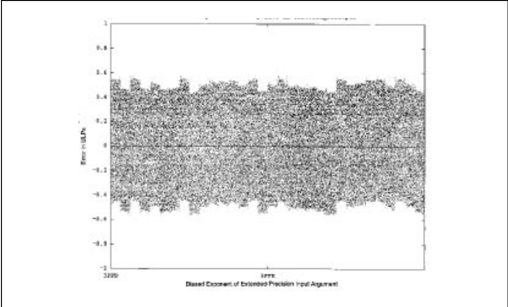
Figure G-21. Scatterplot for F2XM1 (3FFD-3FFE)
