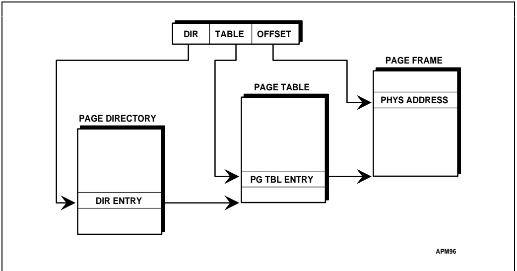
Figure 11-13. Page Translation
