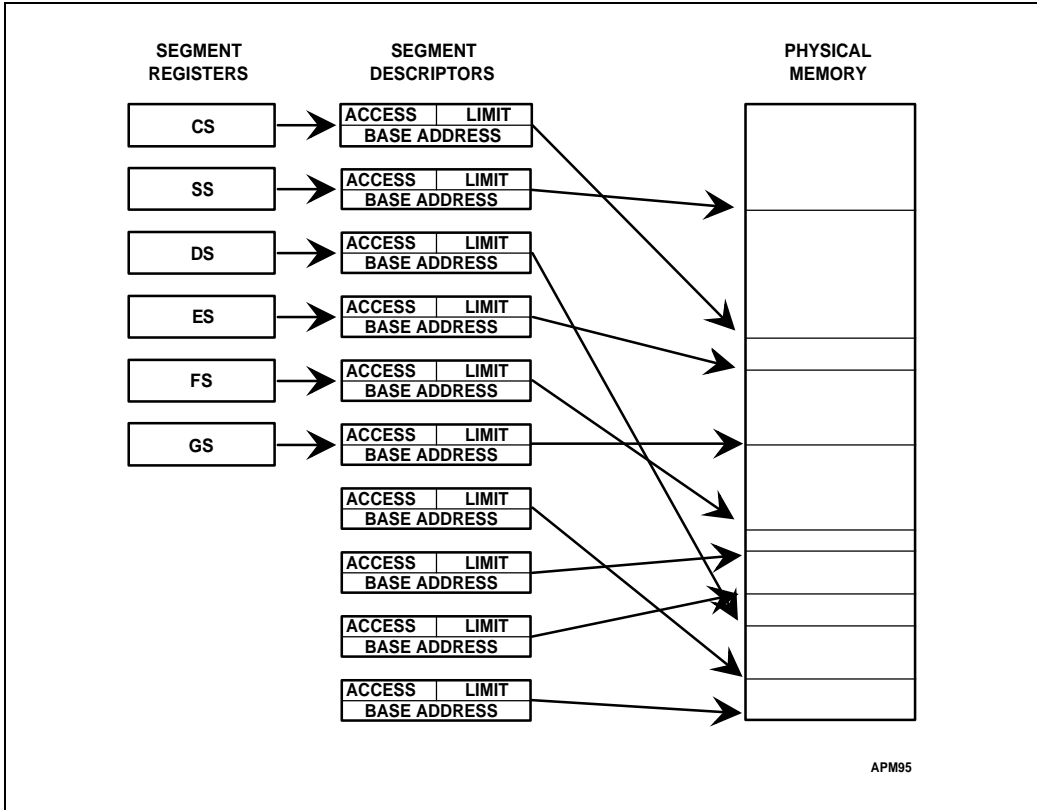
Figure 11-3. Multisegment Model
