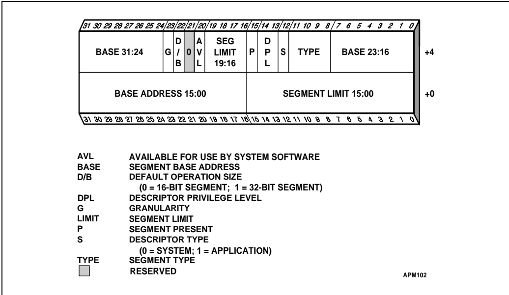
Figure 11-8. Segment Descriptors
