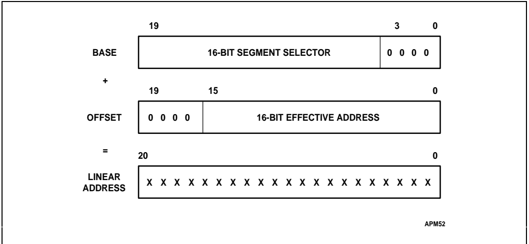
Figure 22-1. 8086 Address Translation
