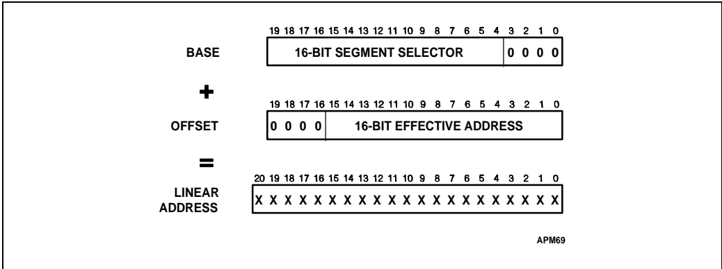
Figure 9-1. 8086 Address Translation
