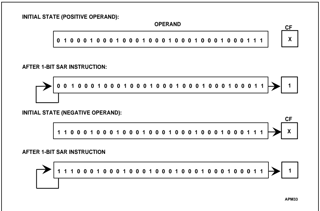
Figure 4-8. SAR Instruction
