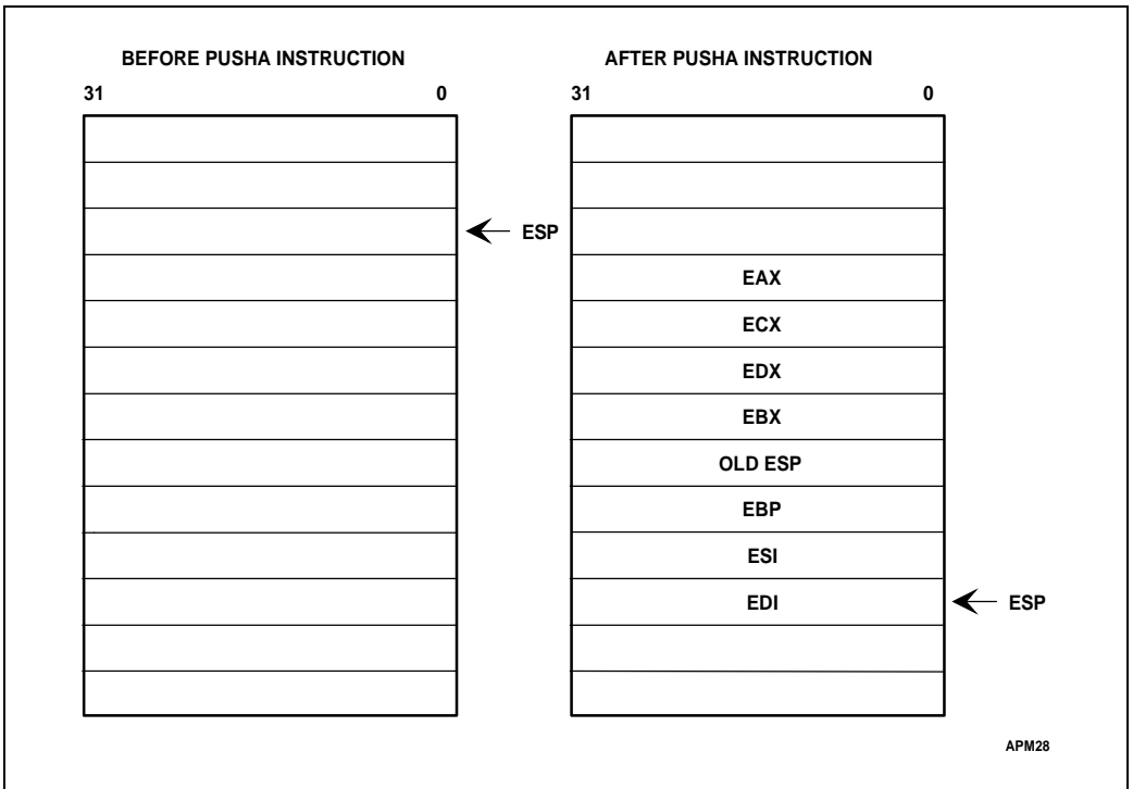
Figure 4-2. PUSHA Instruction
