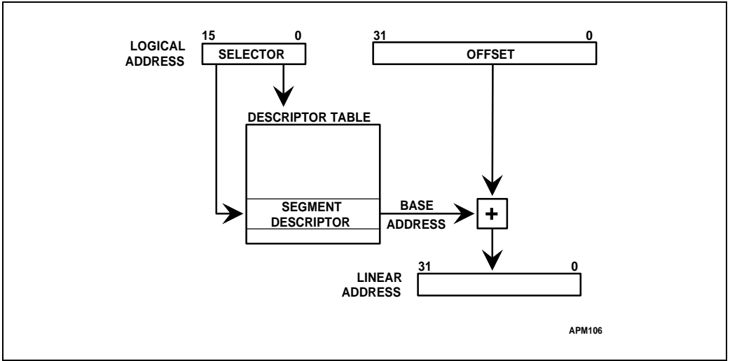
Figure 11-5. Segment Translation
