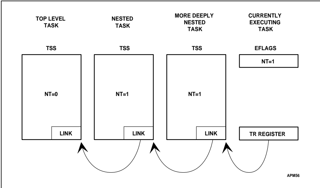
Figure 13-6. Nested Tasks
