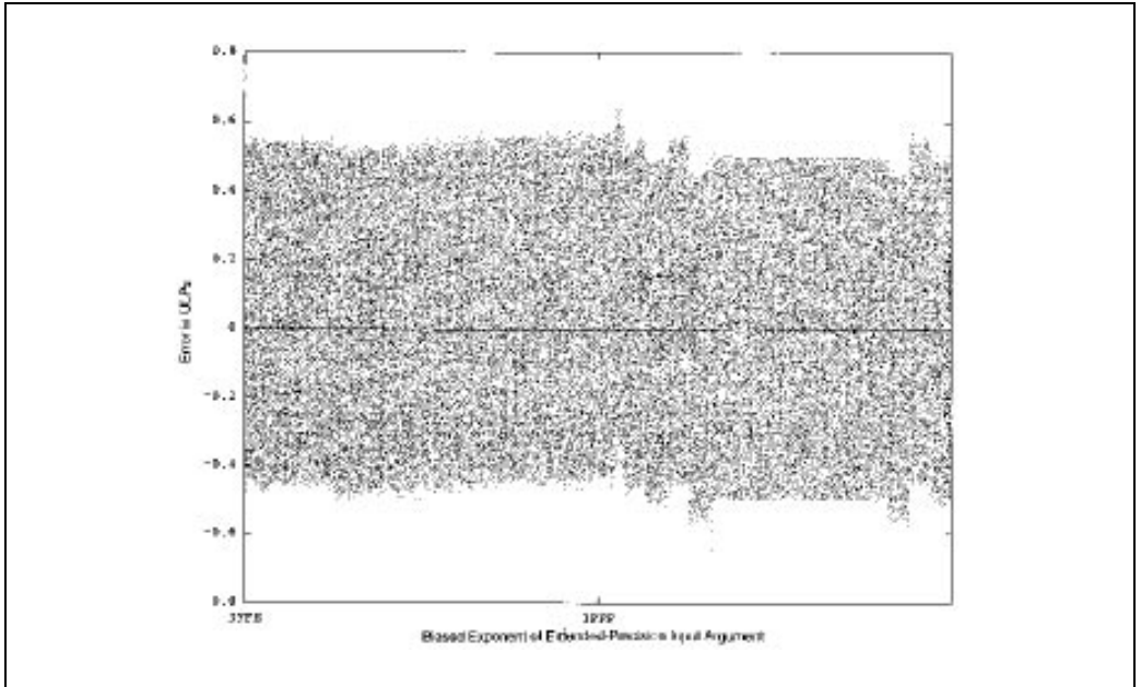
Figure G-7. Scatterplot for FCOS (3FFE-3FFF)
