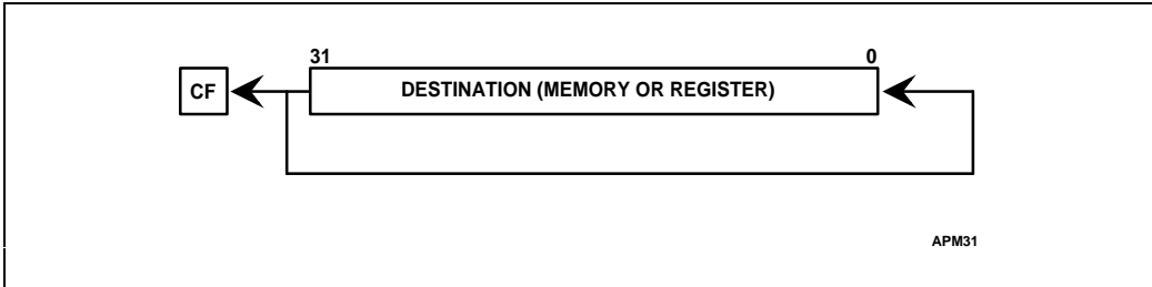
Figure 4-11. ROL Instruction
