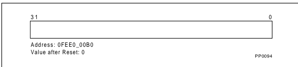
Figure 19-11. EOI Register
