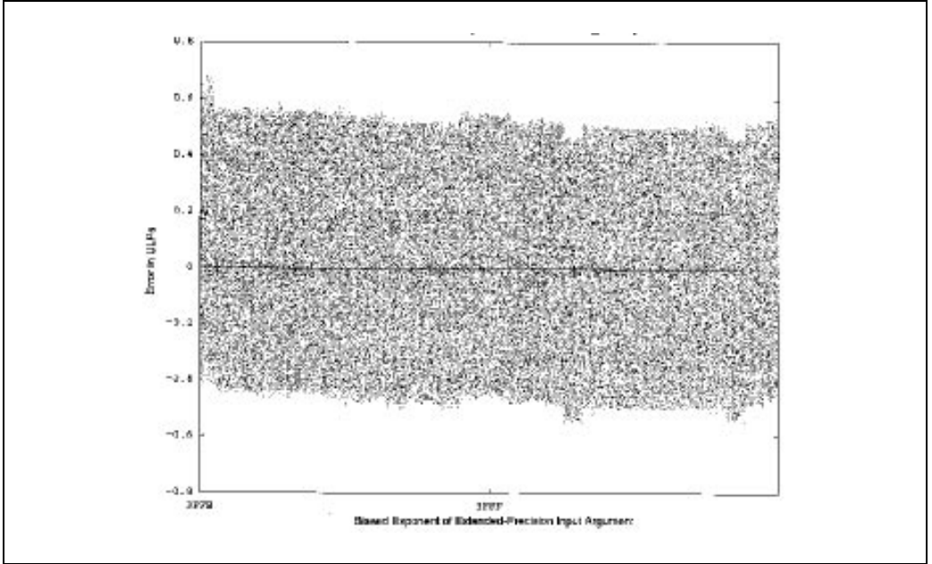
Figure G-3. Scatterplot for FSIN (3FFE-3FFF)
