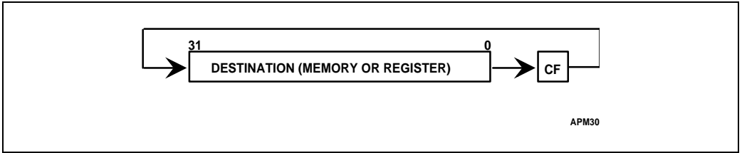
Figure 4-14. RCR Instruction
