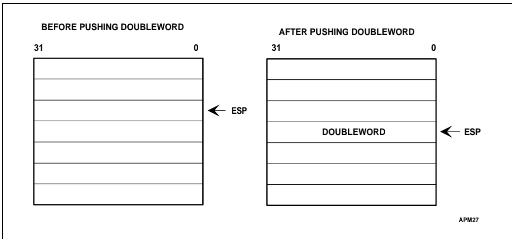
Figure 4-1. PUSH Instruction
