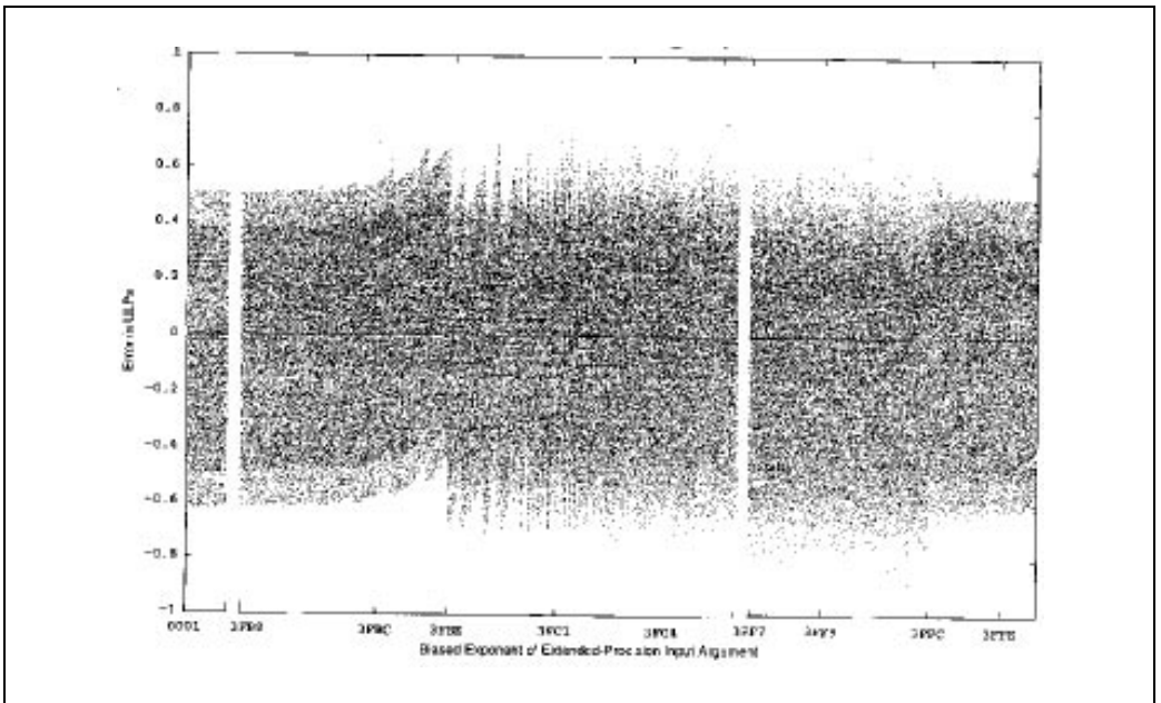
Figure G-16. Scatterplot for FYL2XP1 (0001-3FFE)
