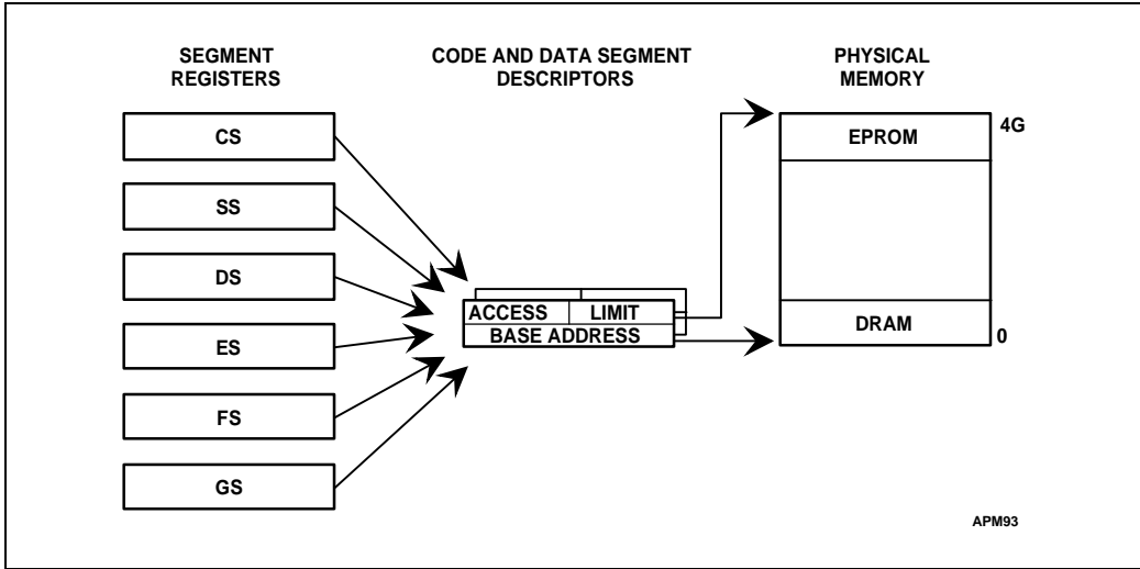
Figure 11-1. Flat Model
