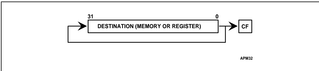
Figure 4-12. ROR Instruction
