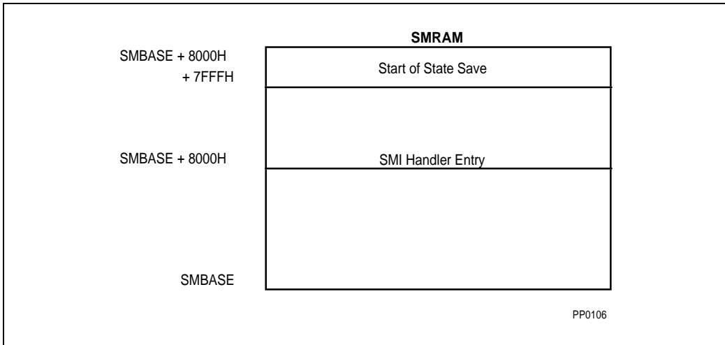
Figure 20-6. SMRAM Usage
