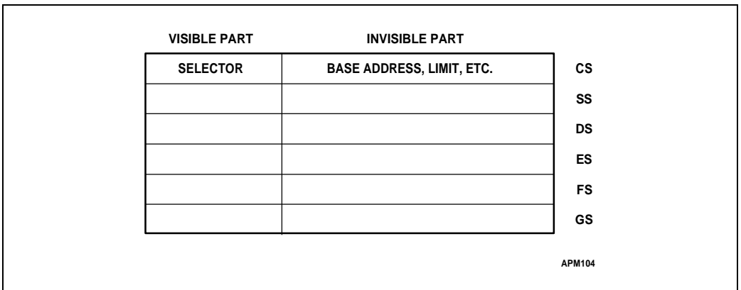
Figure 11-6. Segment Registers
