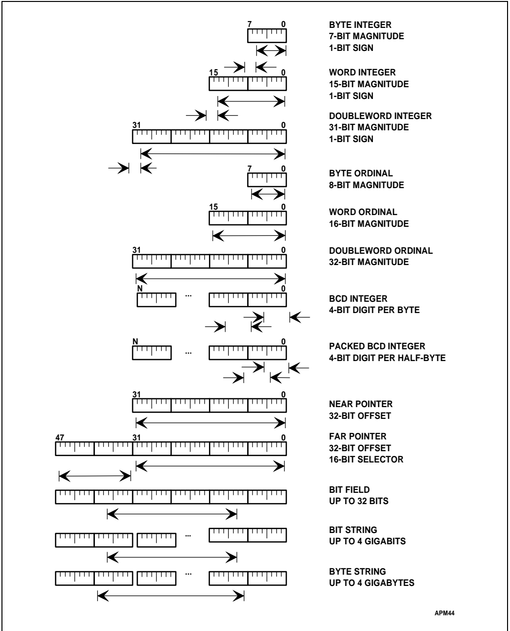
Figure 3-4. Data Types
