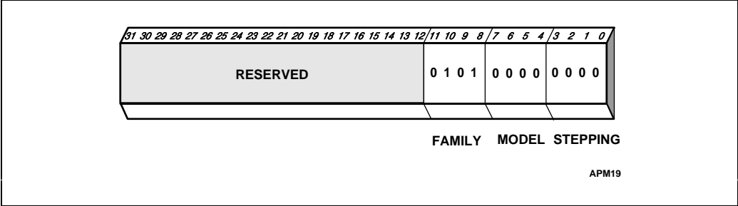
Figure 4-22. EAX Following the CPUID Instruction
