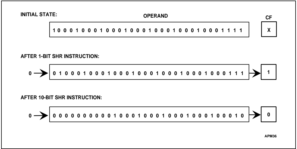
Figure 4-7. SHR Instruction
