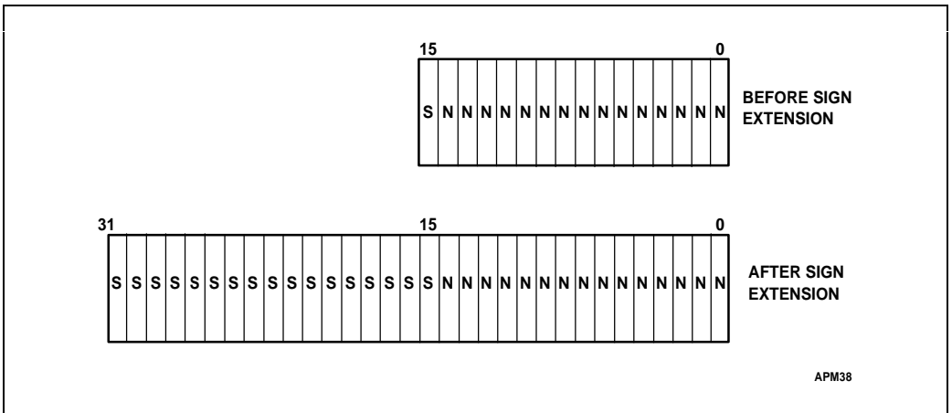
Figure 4-5. Sign Extension
