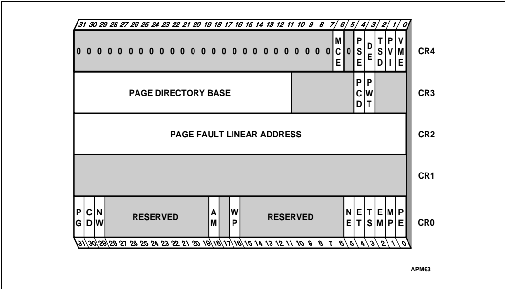
Figure 10-3. Control Registers
