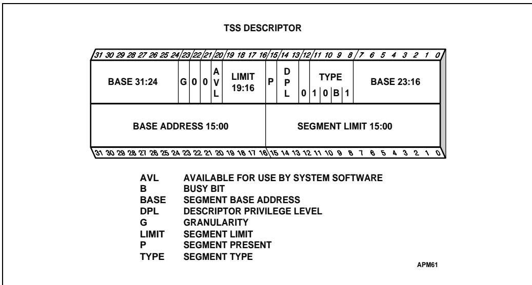
Figure 13-2. TSS Descriptor
