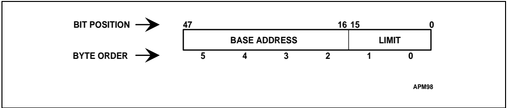
Figure 11-11. Pseudo-Descriptor Format
