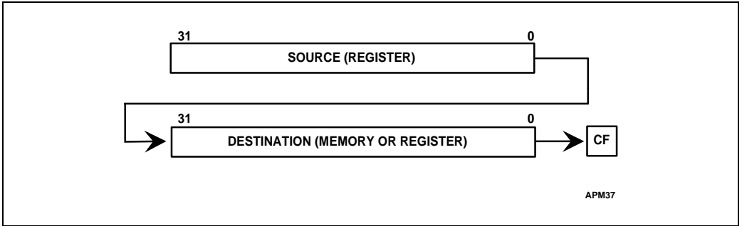
Figure 4-10. SHRD Instruction
