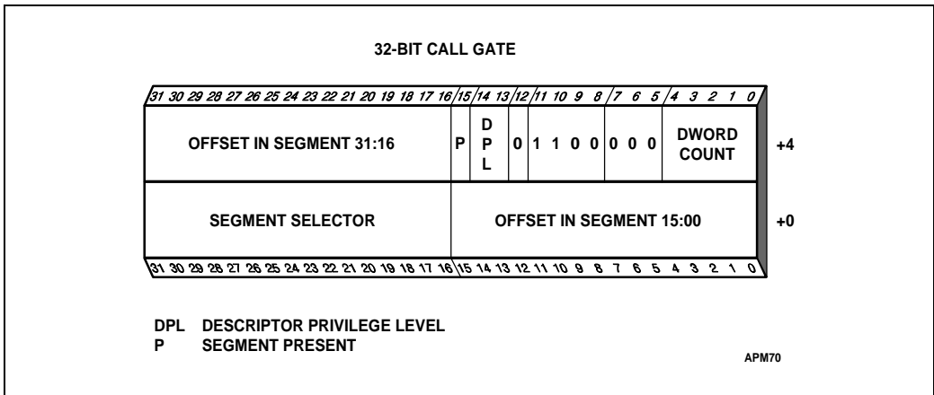
Figure 12-5. Call Gate
